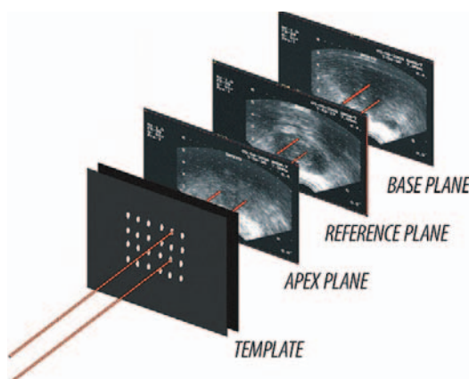
Figure 3. Anatomic plane definition. After image acquisition base, reference and apex planes are defined. Apex refers to the plane that intersects the top of the prostate, while the base is the prostate plane closest to the bladder wall; reference is the middle and the largest cross-section of the gland.
